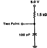
FIGURE 5 — NMOS EQUIVALENT TEST LOAD
