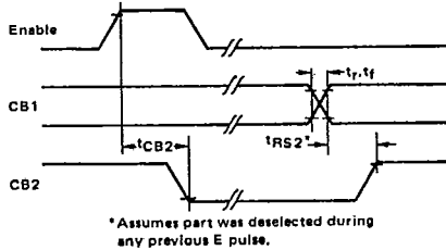
FIGURE 12 - CB2 DELAY TIME (Write Mode; CRB-5=1, CRB-3=CRB-4=0)
