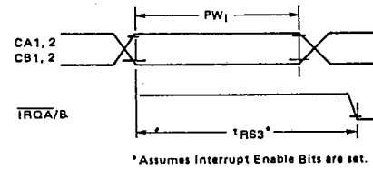
FIGURE 13 - INTERRUPT PULSE WIDTH AND IRQ RESPONSE
