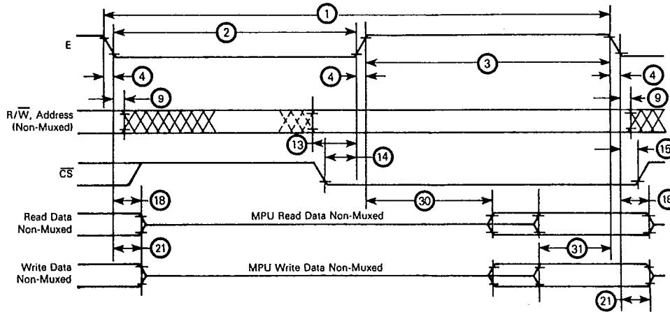
FIGURE 1 — BUS TIMING
