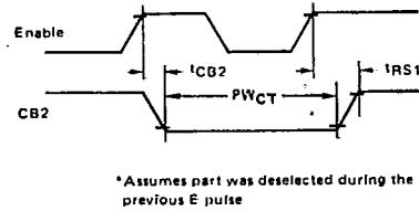
FIGURE 11 - CB2 DELAY TIME (Write Mode; CRB-5=CRB-3=1, CRB-4=0)
