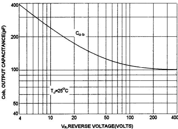
OUTPUT CAPACITANCES
